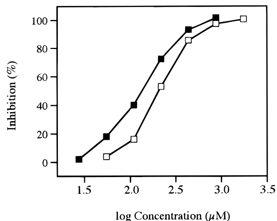
Figure 1. Dose-response curves of ursolic acid ( 1 ) on inhibition of COX-2 (■) and COX-1 (□) catalyzed prostaglandin biosynthesis. Values represent mean \pm S.E.M. ( n = 3-12 ).
